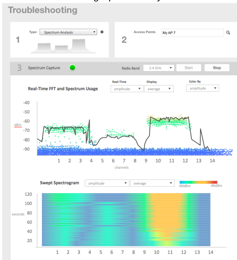
FIGURE 260 Troubleshooting - Spectrum Analysis
