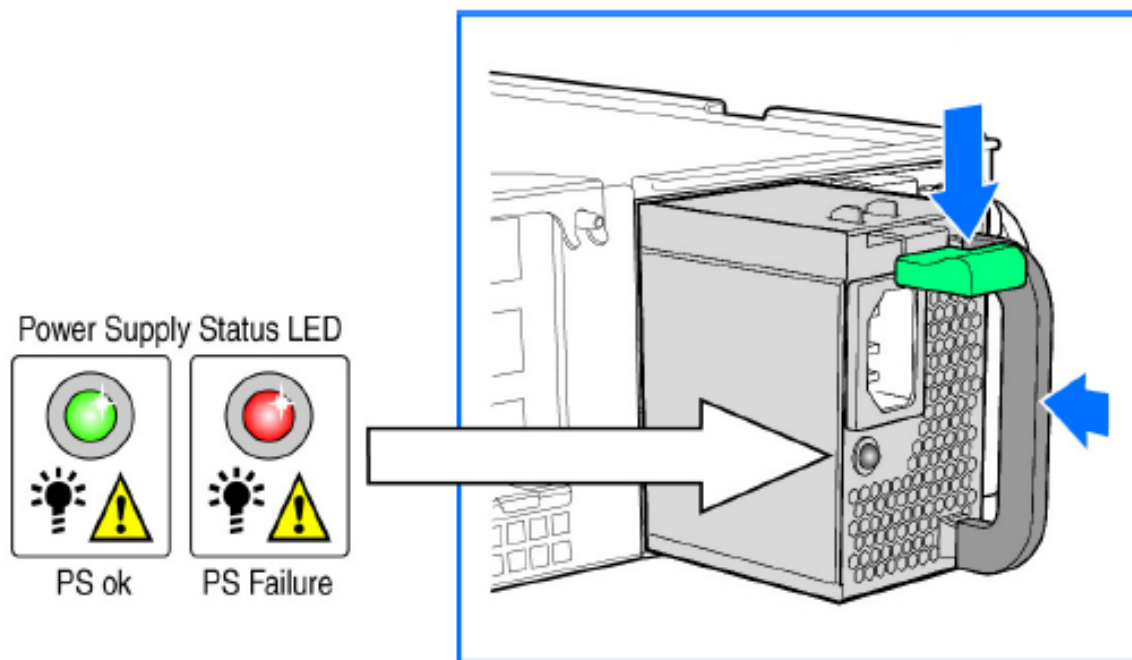
FIGURE 320 Replacing a PSU
