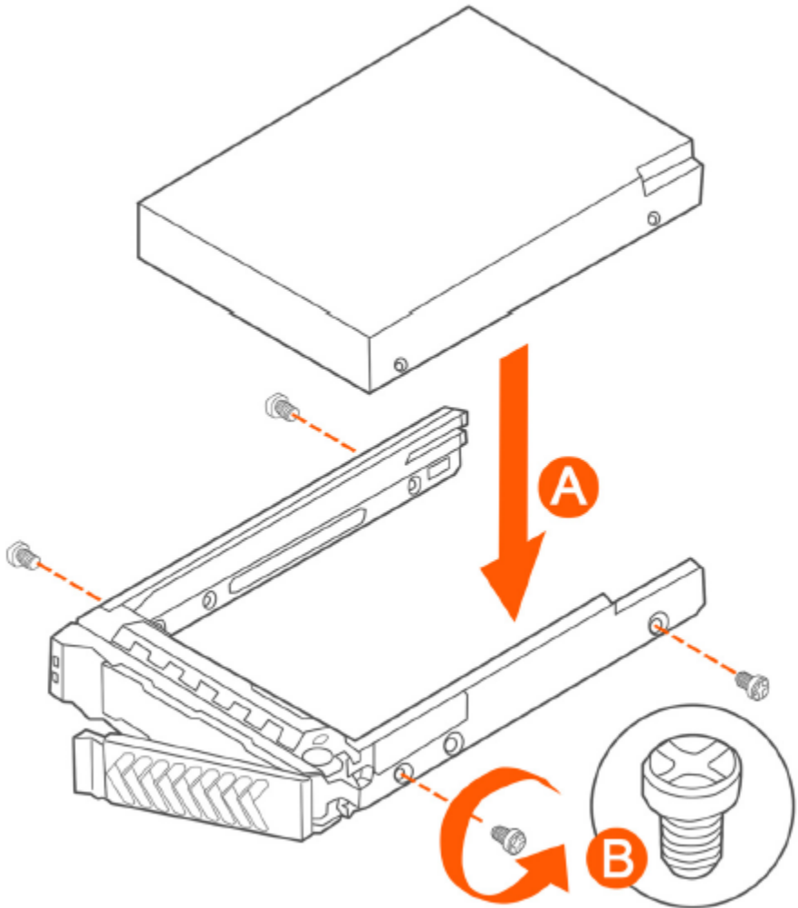
FIGURE 318 Installing the hard drive
